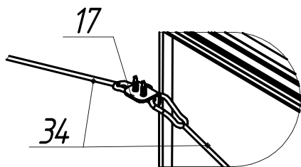
View E
