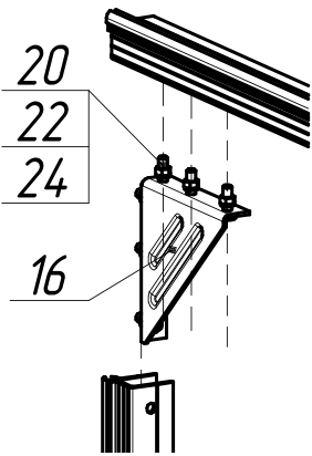
View A
