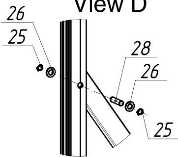
View D
