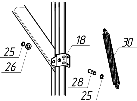
View G
